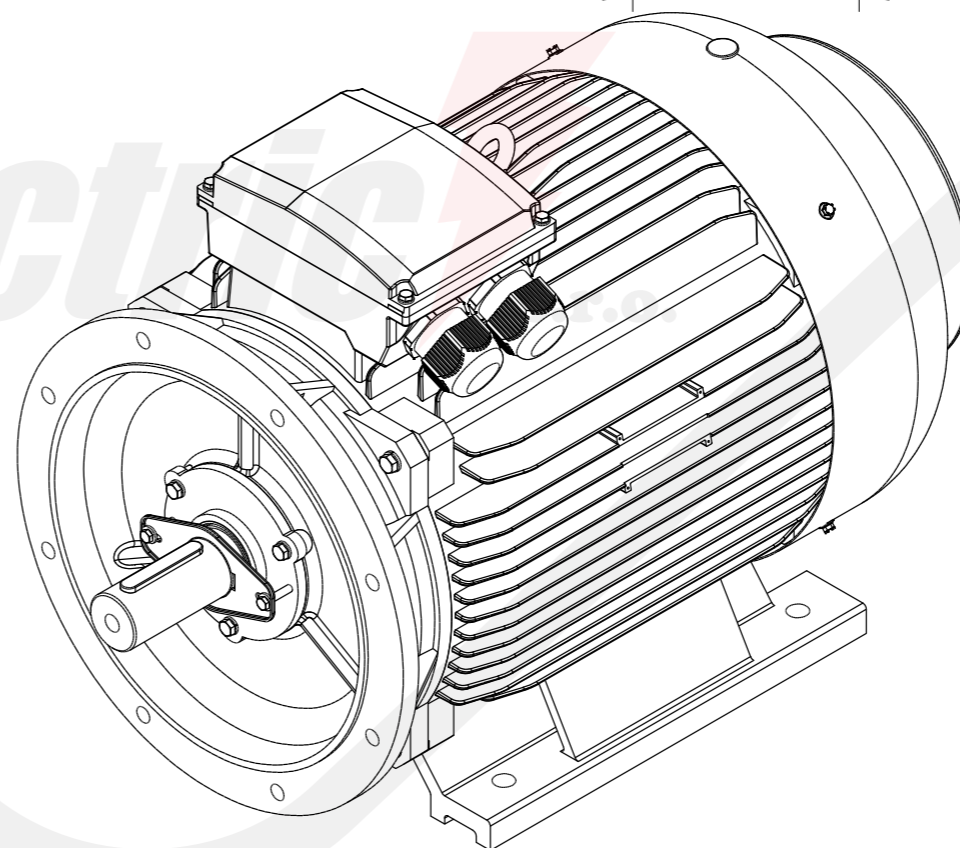
2LC-280M-B35 Mounting diagram
