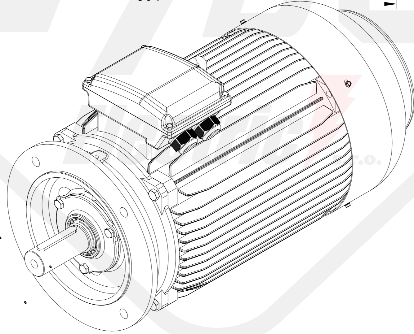
4LC-180L-B5 Mounting diagram
